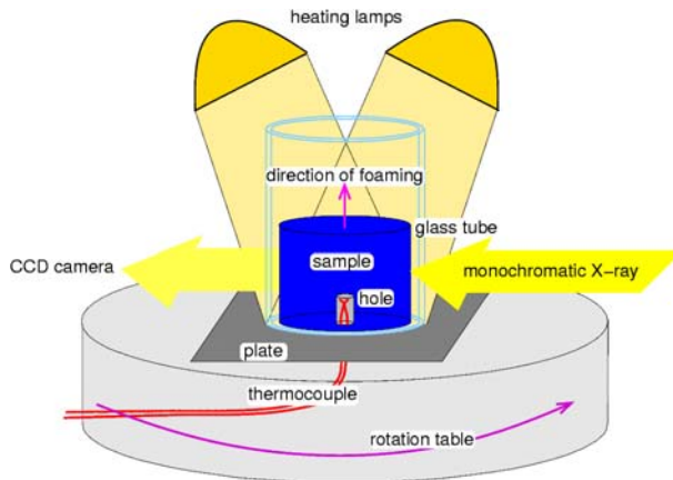
Fig. 2: Heating set up for tomography on liquid foams, consisting of two heating lamps and a sample holder made of a glass tube fixed on refractory clay. The glass tube stabilizes the foam in the liquid state. A thermocouple is located directly inside the sample.
