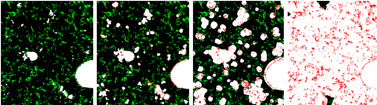
Fig. 10: As an illustration of the dilation algorithm the two Boolean records (white: initial pores, green: SiC particles) of the unfoamed solid aluminium alloy AlSi10Mg are plotted. The initial pores accrue during the production process of the precursor material [3]. The first image shows the starting situation. In the following three pictures the initial pores were blown up and the SiC particle falling in the extended pore volume were counted (red coloured). In the second and the third image the situation after 5 and 10 dilation steps is displayed. The fourth image shows the last dilatation step, where 99% of the sample volume is included.
